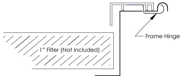
906FG1 Frame Detail
