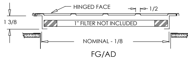
FG/AD Frame Detail
