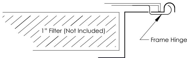
FG/AD Frame Detail
