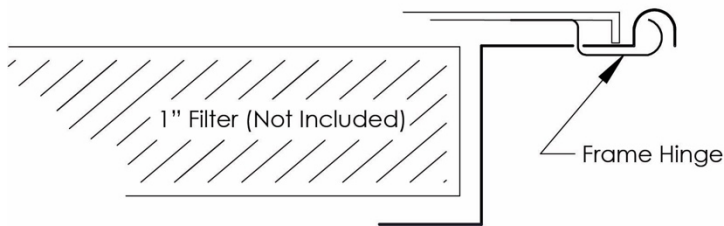
FG/AD Frame Detail
