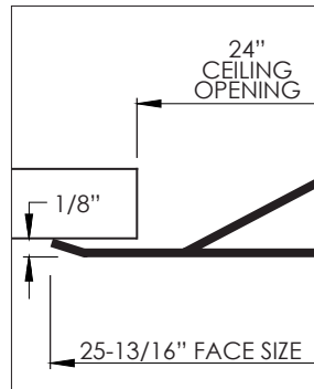
SURFACE MOUNT DETAIL
