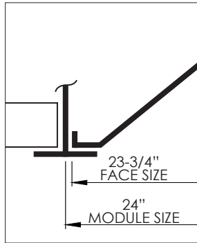
T-BAR MOUNT DETAIL
